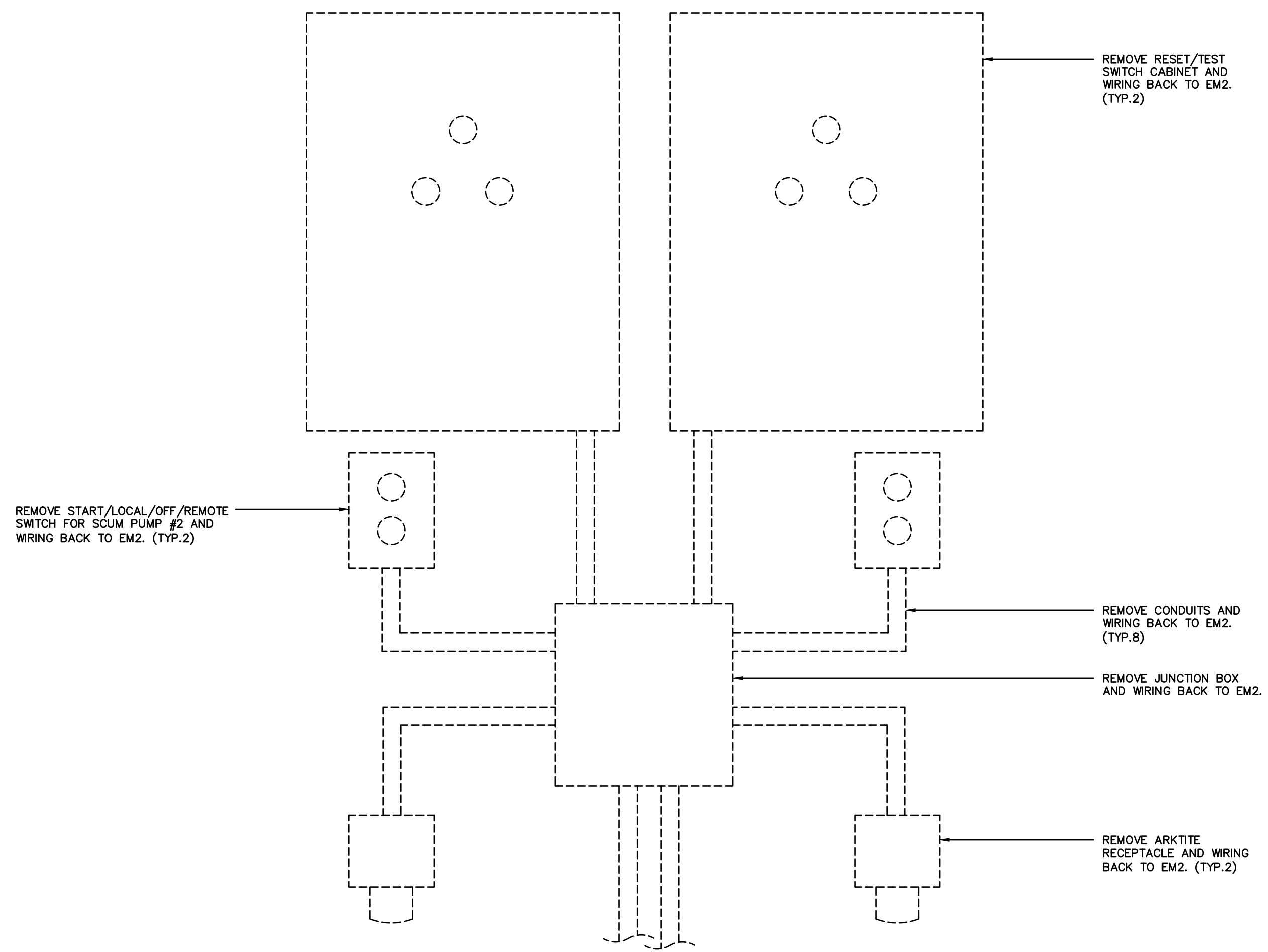
12 ELECTRICAL REMOVALS - SCUM PUMP #2 / RETURN SLUDGE PUMP #2 ELECTRICAL EQUIPMENT E4 SCALE: N.T.S.
