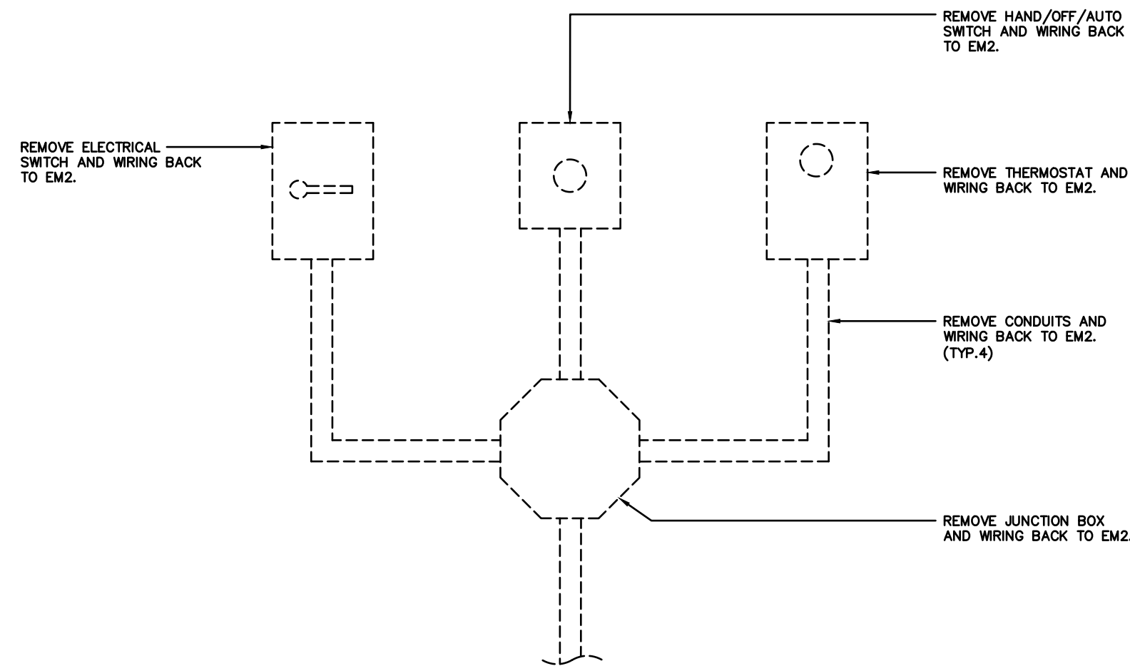
3 ELECTRICAL REMOVALS - CLARIFIER #1/2 ELECTRICAL EQUIPMENT SCALE: N.T.S.
