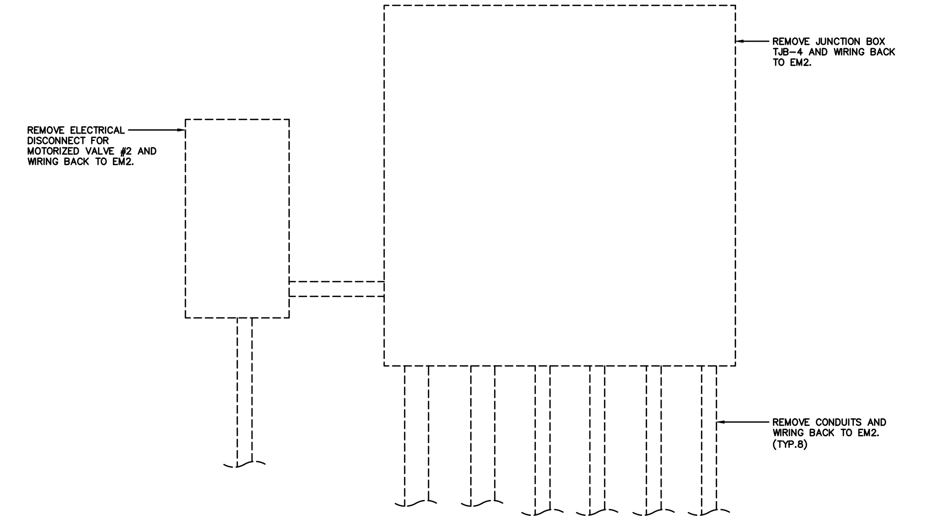
8 ELECTRICAL REMOVALS - MOTORIZED VALVE #2 ELECTRICAL EQUIPMENT SCALE: N.T.S.
