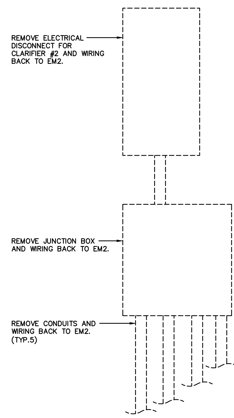
9 ELECTRICAL REMOVALS - CLARIFIER #2 ELECTRICAL EQUIPMENT E3 SCALE: N.T.S.
