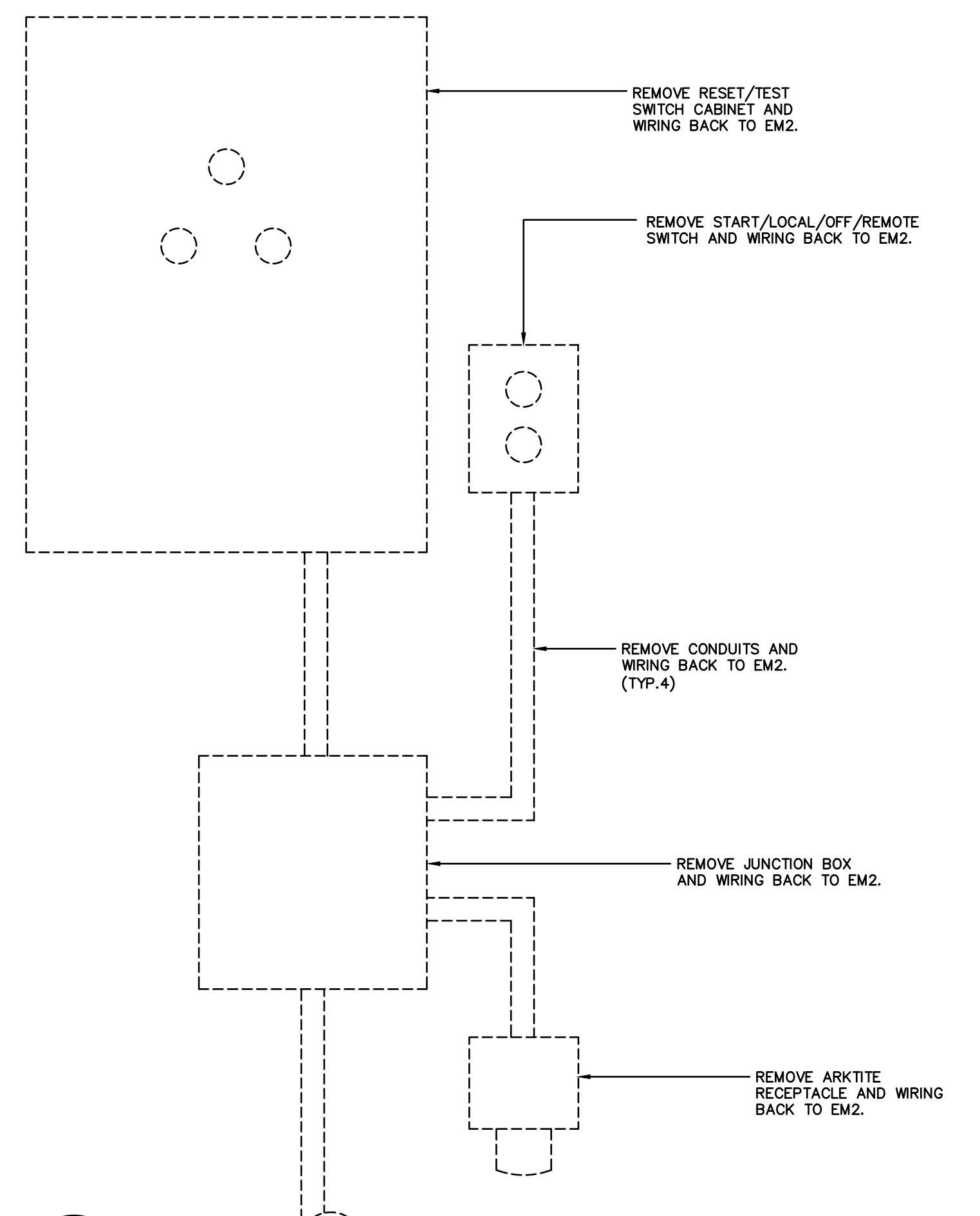
11 ELECTRICAL REMOVALS - SLUDGE REMOVAL PUMP #2 ELECTRICAL EQUIPMENT E4 SCALE: N.T.S.
