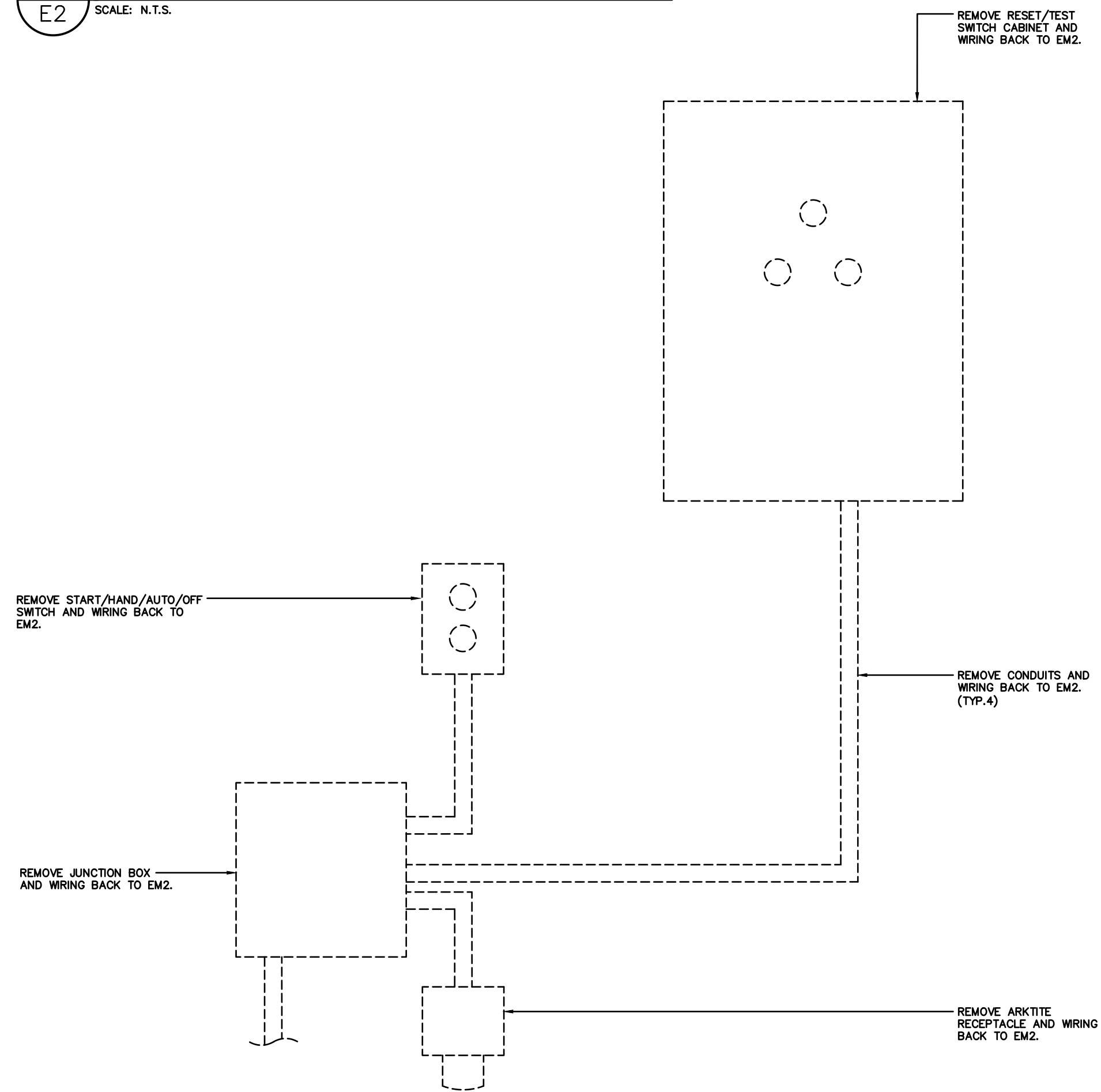
4 ELECTRICAL REMOVALS - SCUM PUMP ELECTRICAL EQUIPMENT SCALE: N.T.S.
