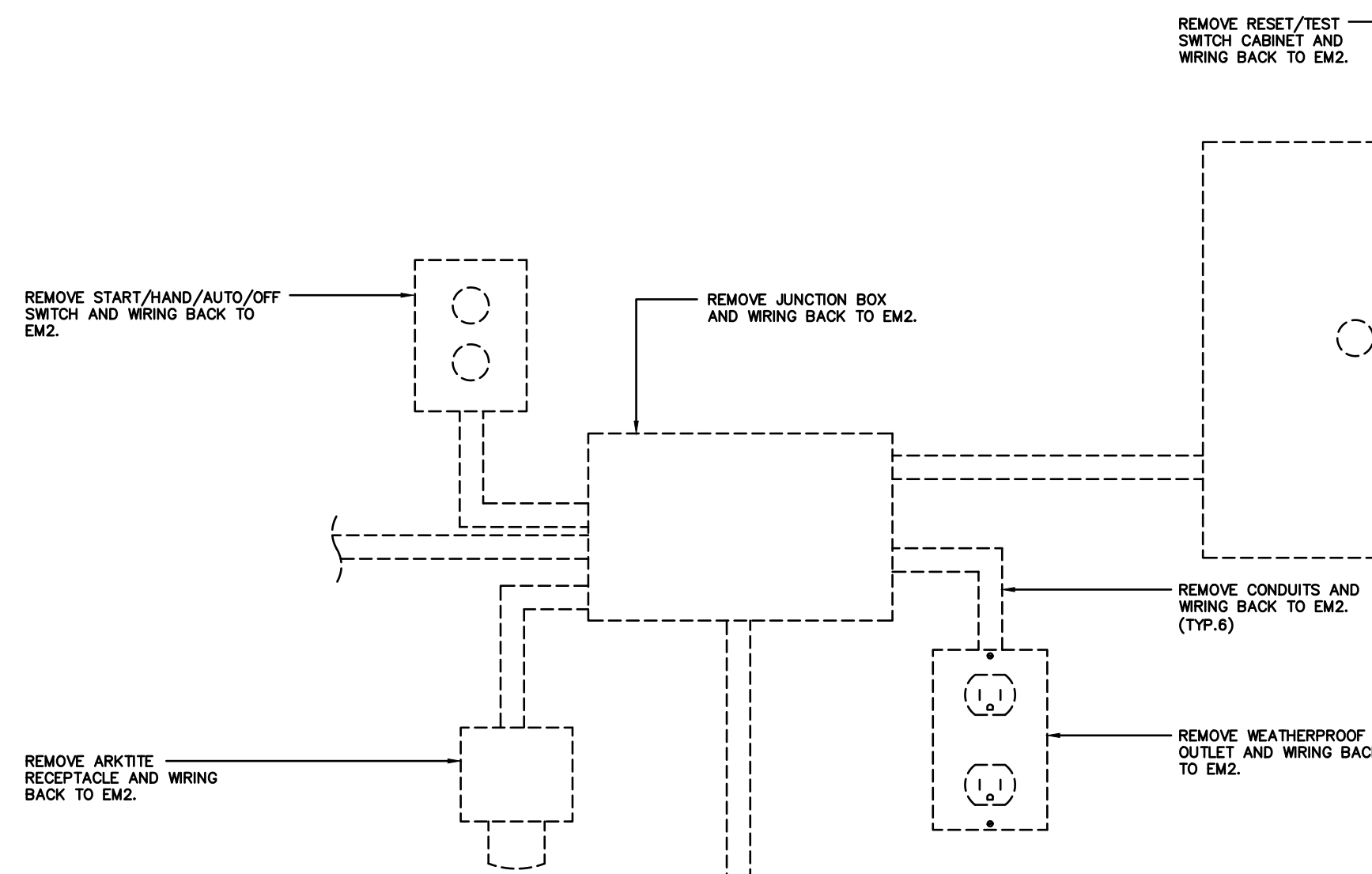
7 ELECTRICAL REMOVALS - SLUDGE PUMP ELECTRICAL EQUIPMENT SCALE: N.T.S.
