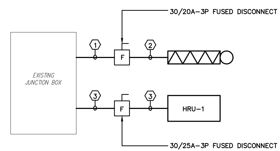
PARTIAL SINGLE LINE DIAGRAM - ELECTRICAL RENOVATION SCALE: N.T.S
