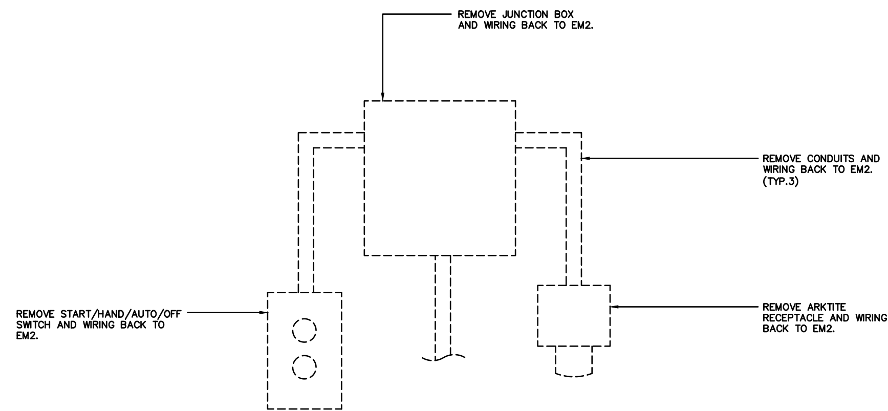
6 ELECTRICAL REMOVALS - ELECTRICAL EQUIPMENT SCALE: N.T.S.
