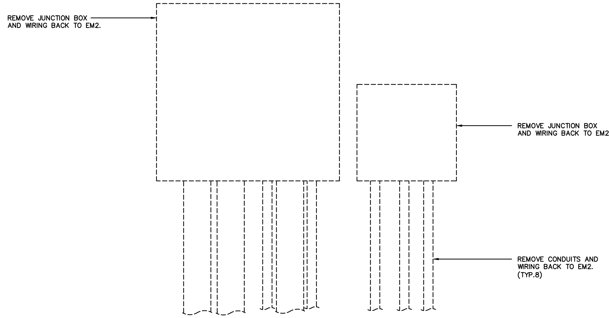
13 ELECTRICAL REMOVALS - JUNCTION BOXES FOR CLARIFIER #2 E4 SCALE: N.T.S.
