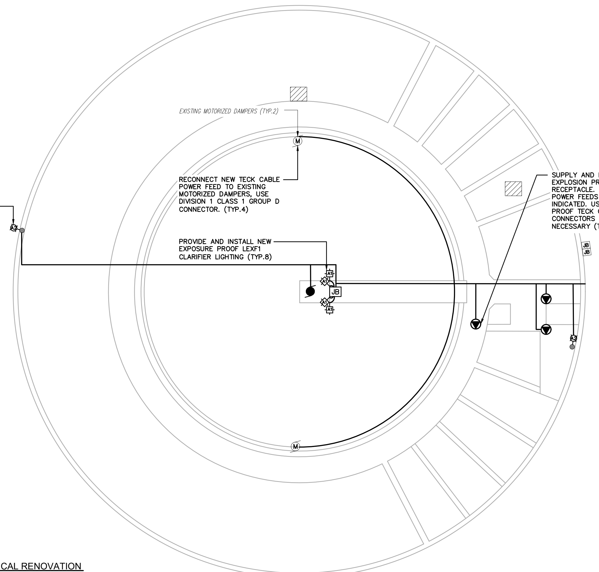
CLAIRIFIER #1- ELECTRICAL RENOVATION SCALE: N.T.S.
