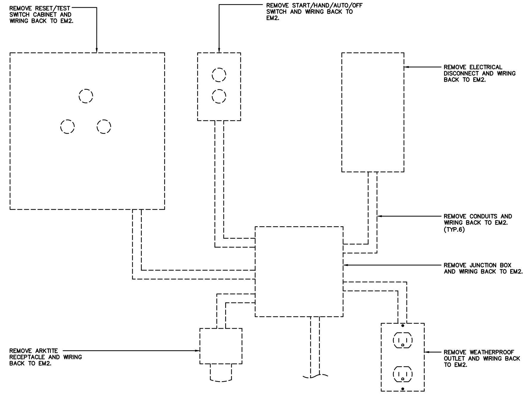
5 ELECTRICAL REMOVALS - MOTORIZED VALVE #1 ELECTRICAL EQUIPMENT SCALE: N.T.S.
