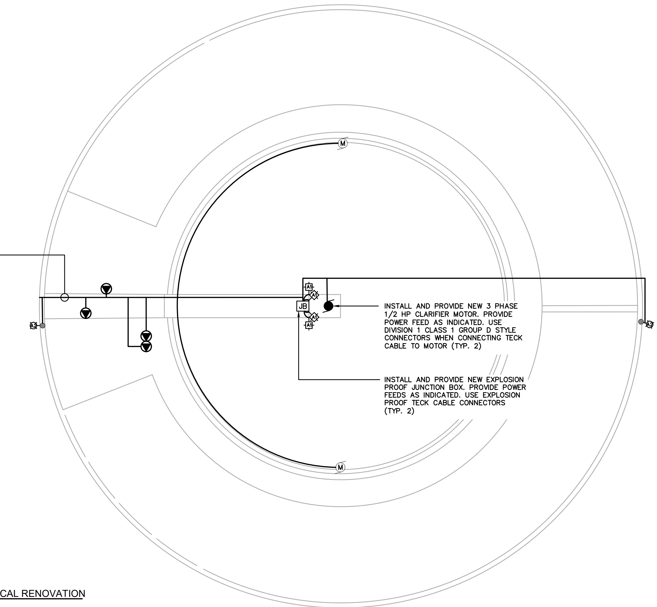
CLAIRIFIER #1- ELECTRICAL RENOVATION SCALE: N.T.S.
