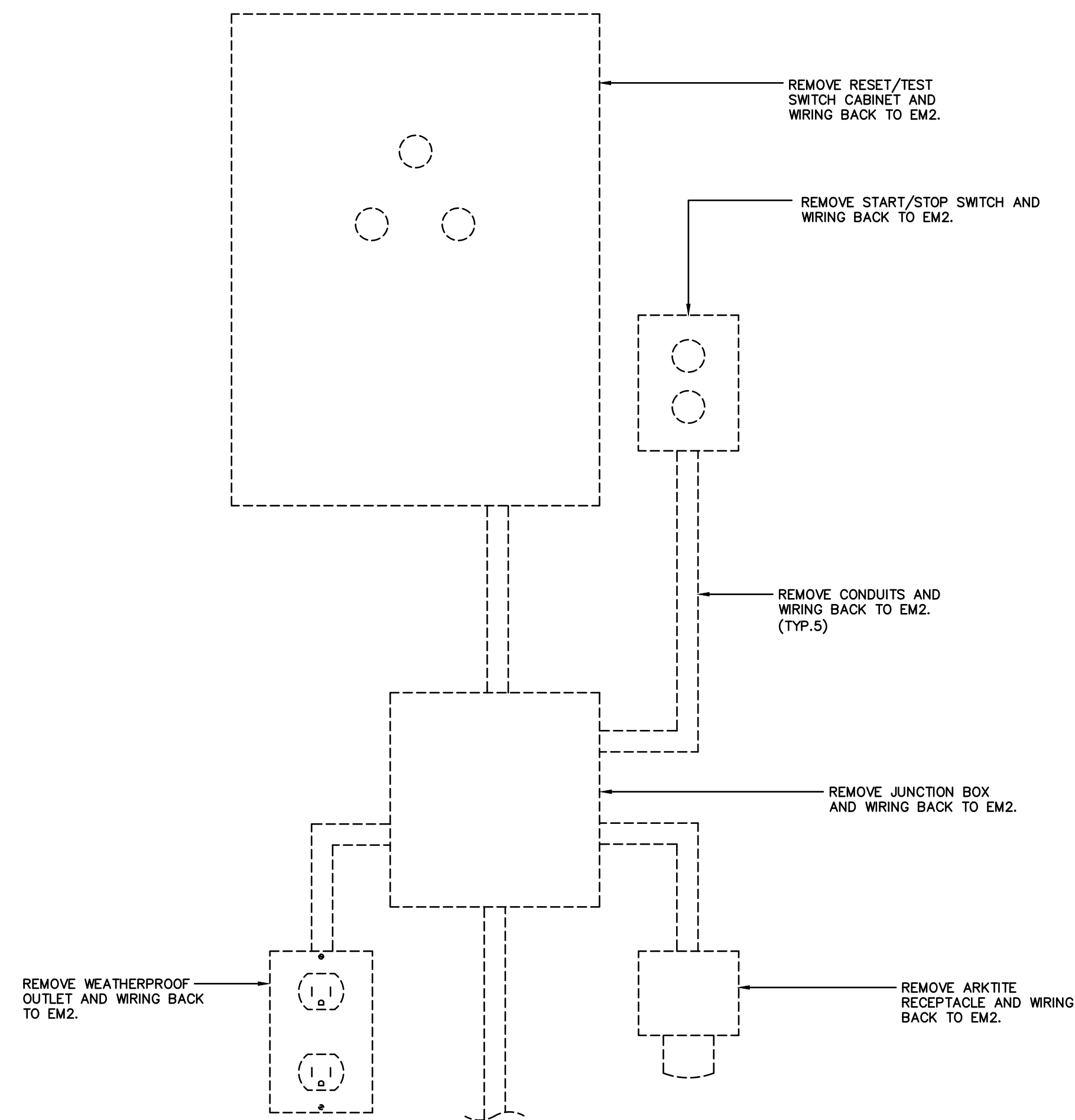
10 ELECTRICAL REMOVALS - SUPERNATANT PUMP #2 ELECTRICAL EQUIPMENT E4 SCALE: N.T.S.
